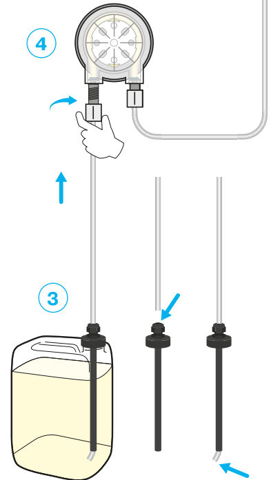
Suction kit for 20 l canister #13415
