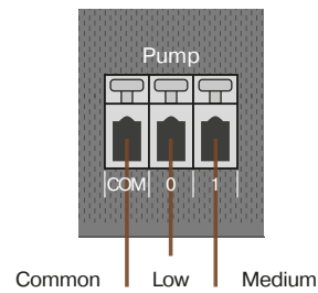
VS filtration pump Pentair, Dab, Speck – newer types
