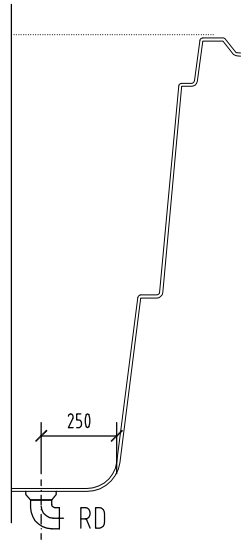
DETAIL M 1:25
